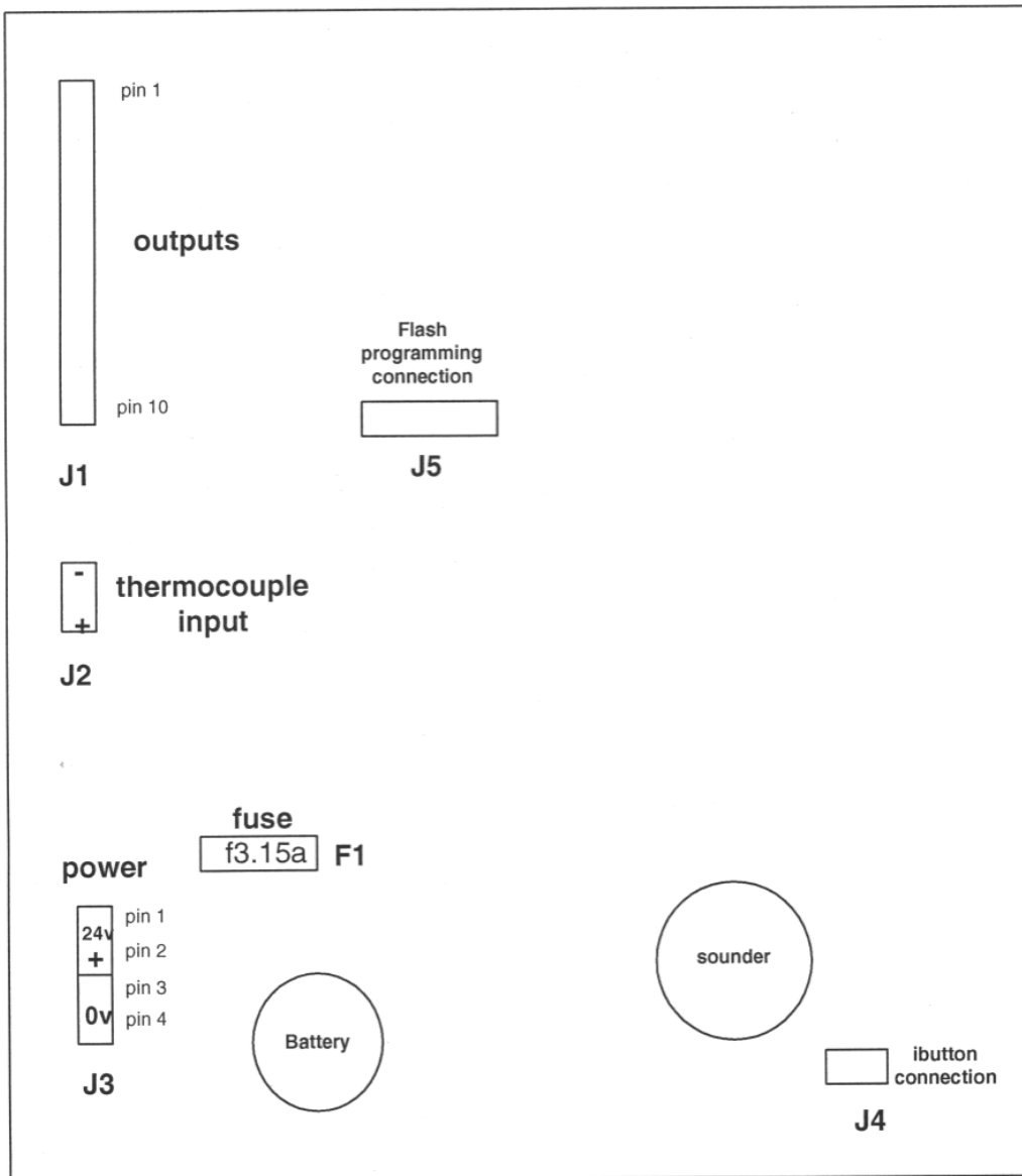
Figure 11: Controller layout
