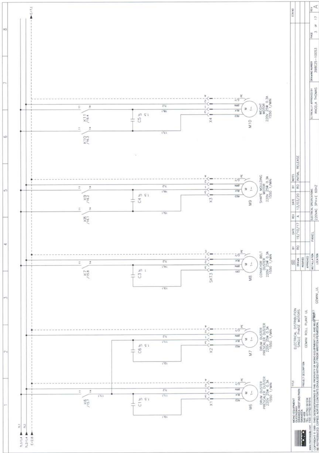
Figure 14.3: Drawing No. 398E2510053 (3 of 17)
