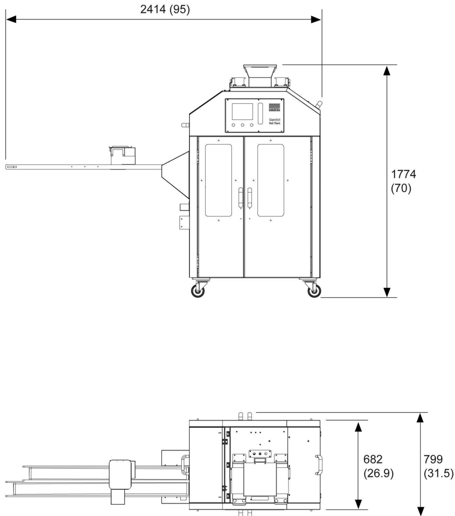
Figure 2.1: Dimensions without the roll forming unit
