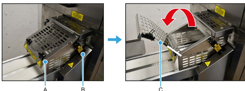
Figure 4.1: Opening the Offtake conveyor guard
