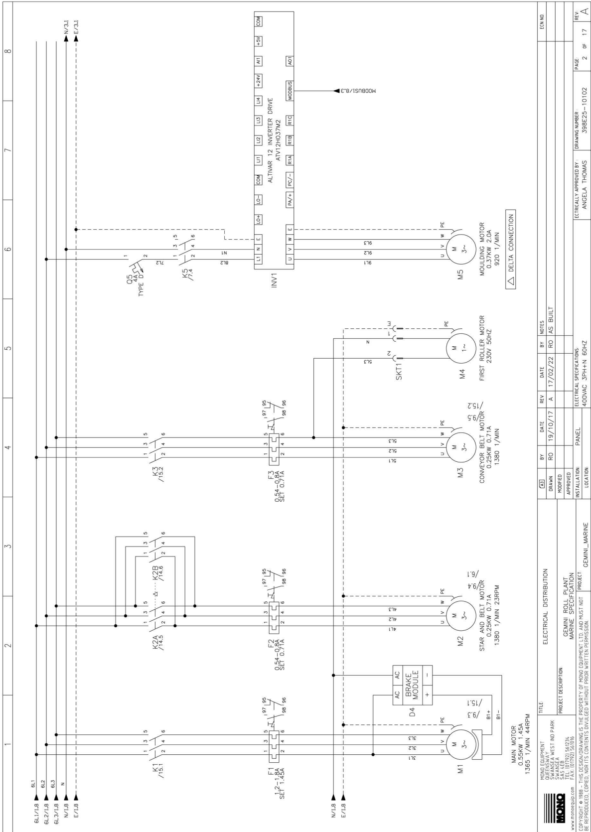
Figure 14.2: Drawing No. 398E2510102 (2 of 17)
