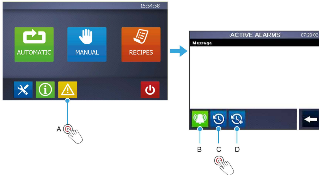
Figure 7.8: Active Alarms screens
