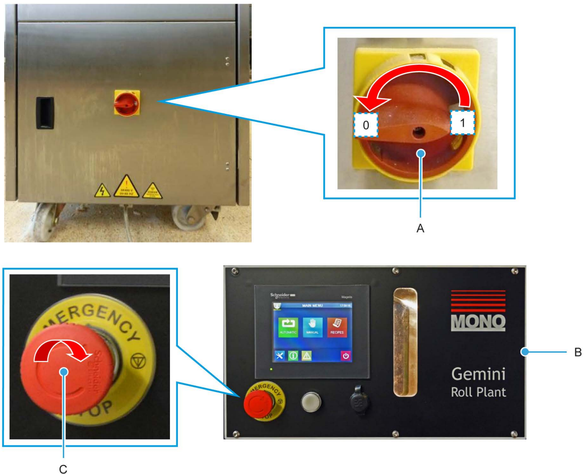
Figure 6.1: Emergency stop buttons
